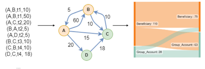
Fig. 3. An example outlining the proposed methodology. Starting from the transactions, in format (sender, receiver, amount, timestamp), we filter them on the timestamps to obtain a subset for the time period of interest. Then, we construct the transaction network. Relying on the weights and attributes of the transaction network, we can aggregate to construct the Sankey diagrams. In the example of the transaction network, nodes are colored according to the type, while the weights on links correspond to the amount of tokens flowing from the source to the destination.
